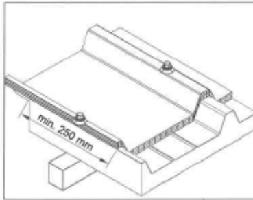
compensation seals
