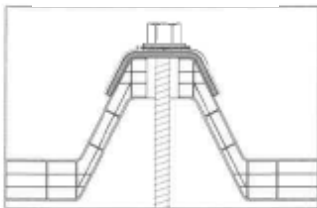
CAP FASTENING
